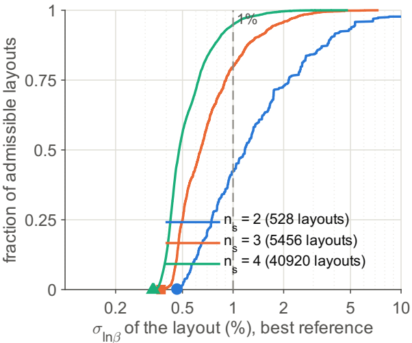
(a) Placement sensitivity (LSM6DSV16X)
